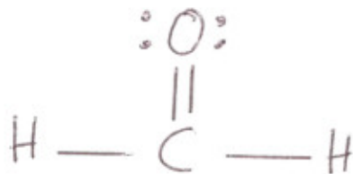
j) \text{CH}_2\text{O} (C is the central atom)
