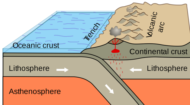
Convergent plate boundary between a oceanic plate and continental plate. From Creative Commons (CC).
