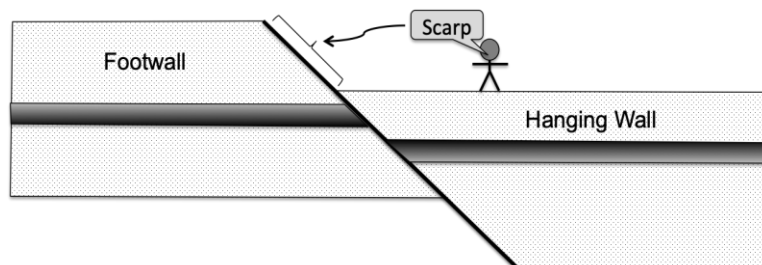
Cross-section perspective drawing of a normal fault.
