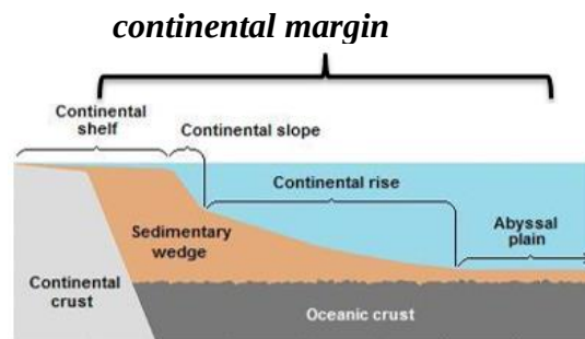
Passive continental margin. –CC
