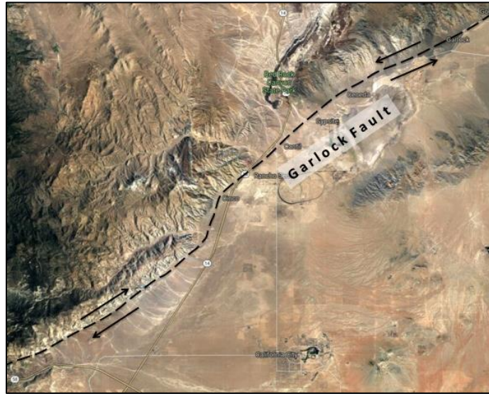
The trace of the Garlock fault. Note CA-14 and Red Rock Canyon. – Google Earth.
