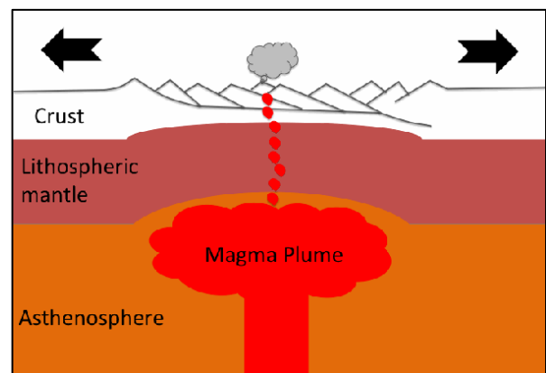
Tensional stresses initiating a divergent boundary within continental crust.
