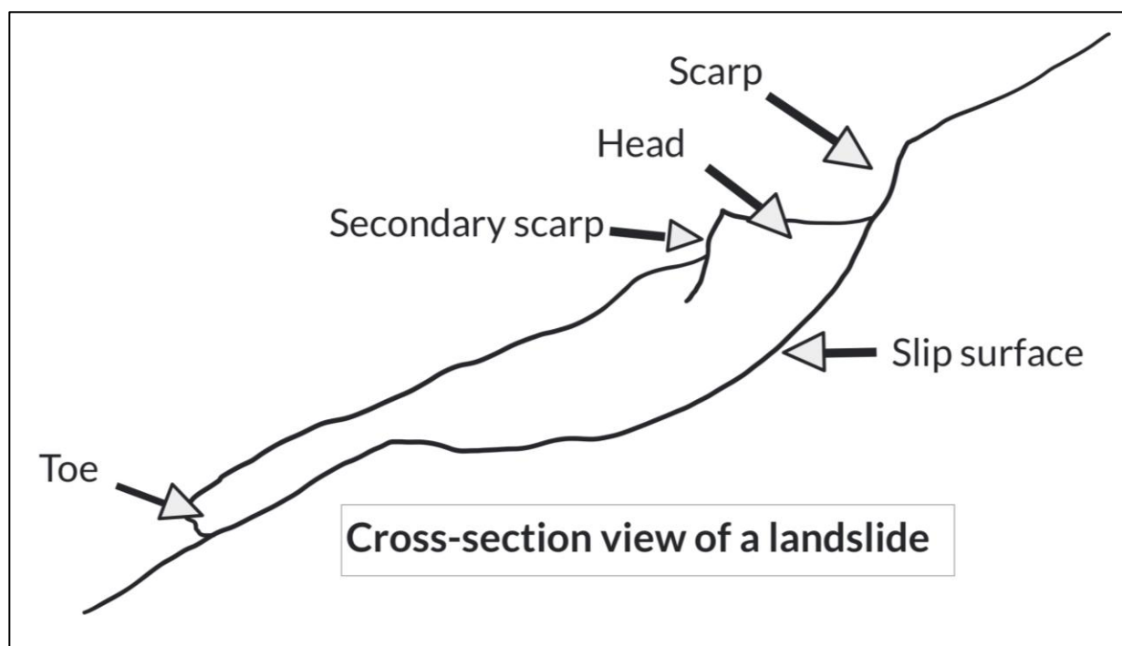
Cross-section view of landslide.
