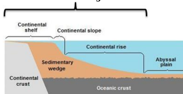
Passive continental margin –CC.
