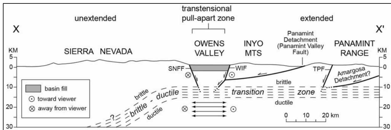
Cross-section from the Sierra Nevada mountain range to the Panamint mountain range. SNFF = Sierra Nevada Frontal fault; WIF = White Inyo Fault. Circled \square indicates crust moving away from viewer, while the bullseye symbol indicates crust moving towards. From Stevens et al 2013.
